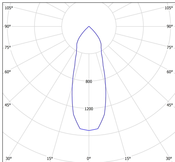
cd/klm \eta = 92\% — C0 - C180 — C90 - C270
