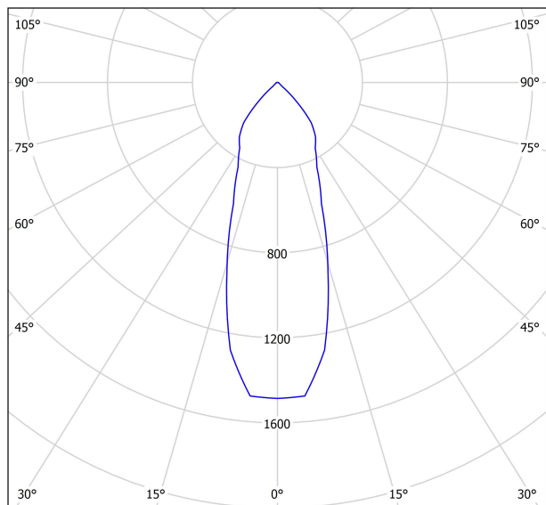
cd/klm — C0 - C180 — C90 - C270 η = 92%
