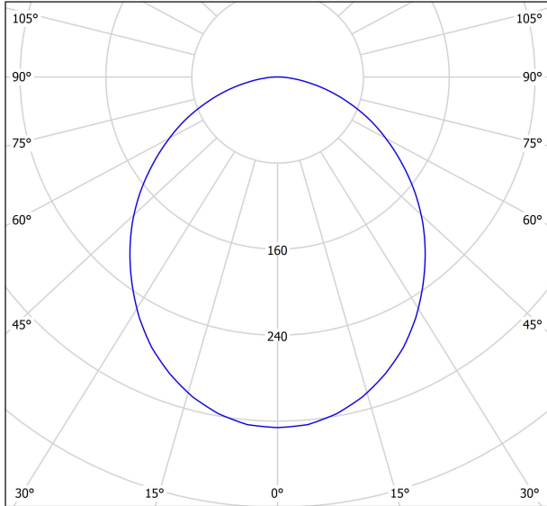
cd/klm \eta = 83\% — C0 - C180 — C90 - C270
