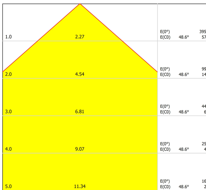
Distance [m] Cone Diameter [m] Illuminance [lx] — C0 - C180 (Half-value Angle: 97.2°)
