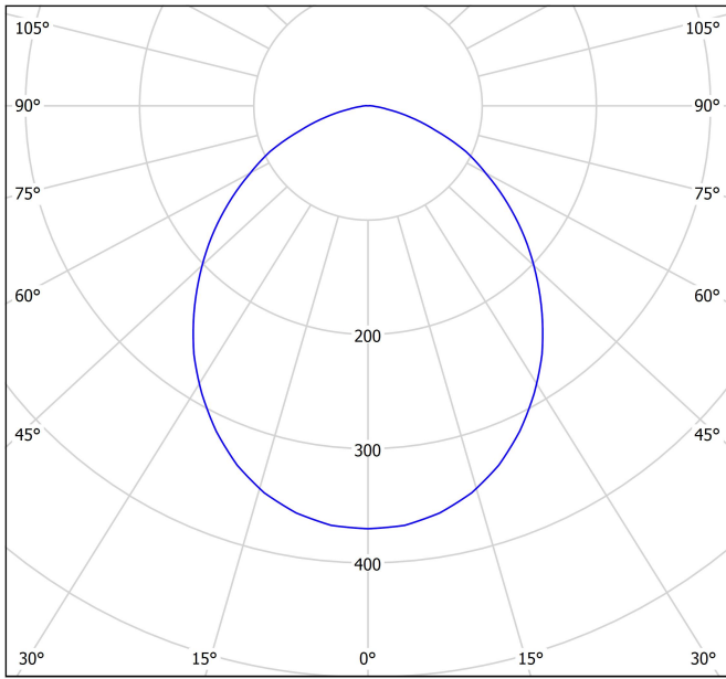
cd/klm — C0 - C180 — C90 - C270 η = 88%
