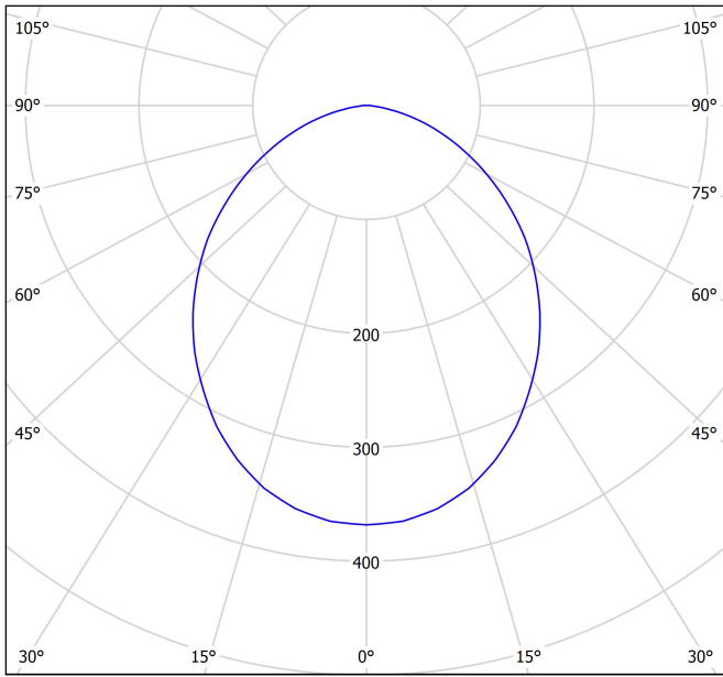
cd/klm — C0 - C180 — C90 - C270 η = 89%
