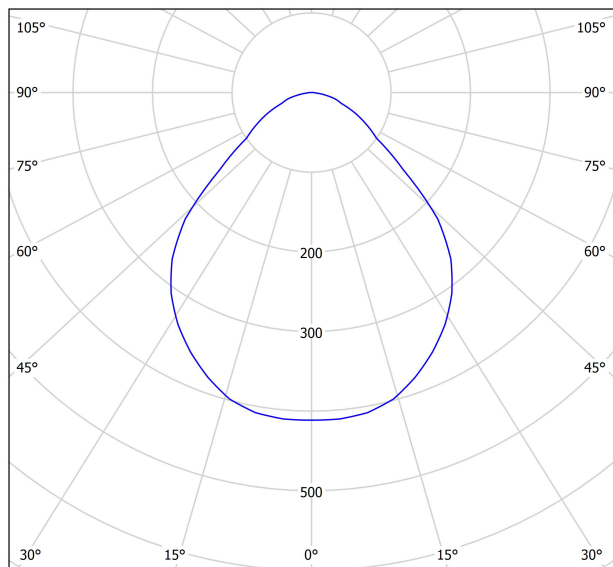
cd/klm — C0 - C180 — C90 - C270 η = 87%
