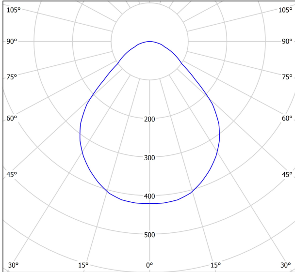
cd/klm \eta = 89\% — C0 - C180 — C90 - C270
