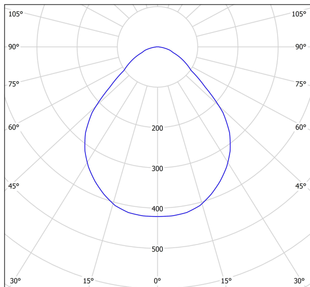
cd/klm — C0 - C180 — C90 - C270 η = 89%
