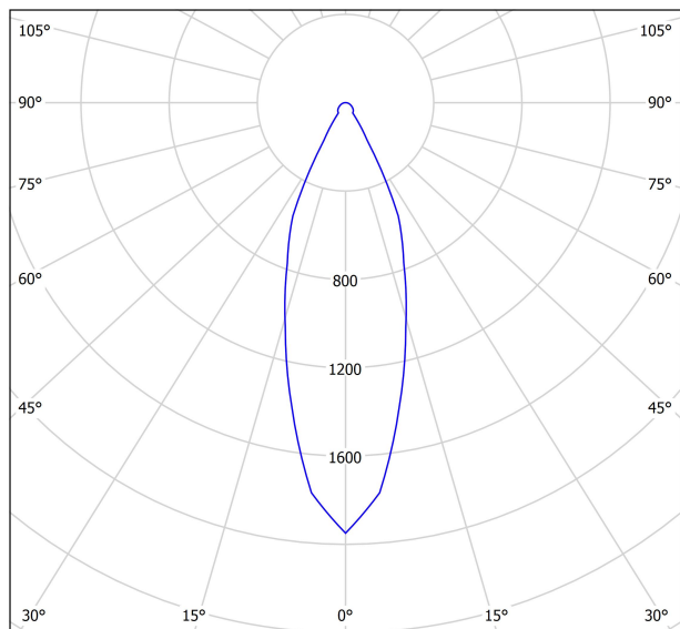
cd/klm — C0 - C180 — C90 - C270 η = 86%
