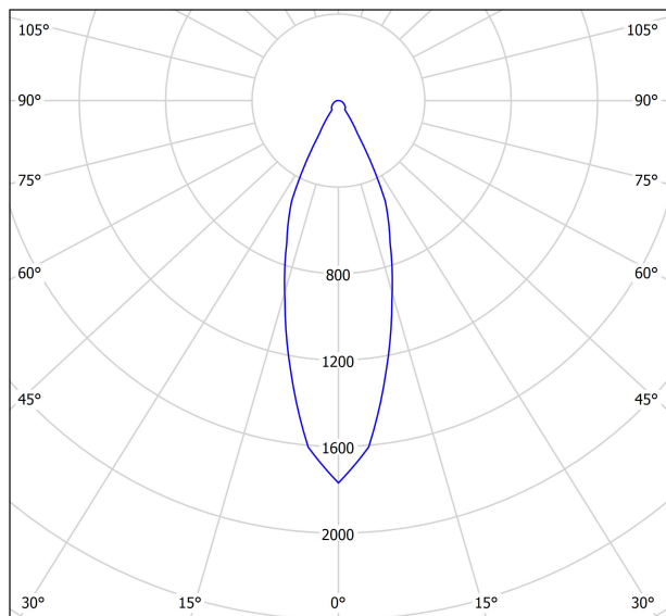
cd/klm — C0 - C180 — C90 - C270 η = 78%
