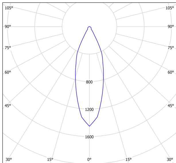
cd/klm — C0 - C180 — C90 - C270 η = 64%
