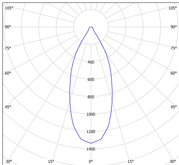
cd/klm — C0 - C180 — C90 - C270 η = 77%
