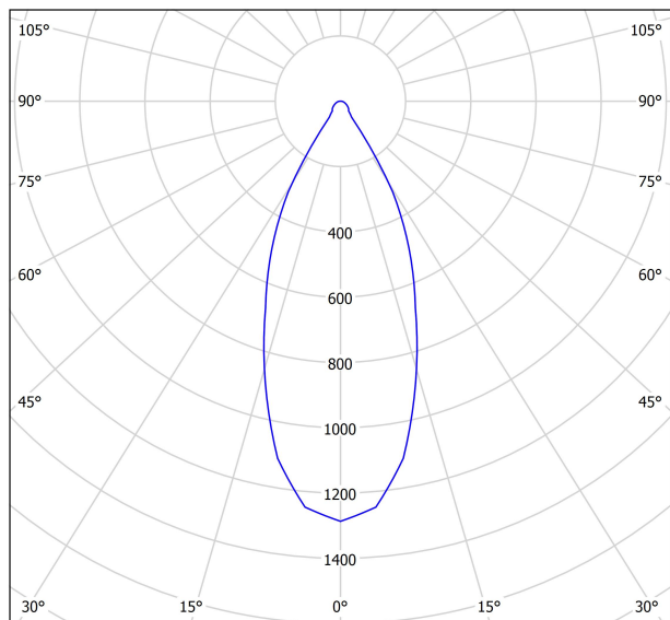
cd/klm — C0 - C180 — C90 - C270 η = 74%
