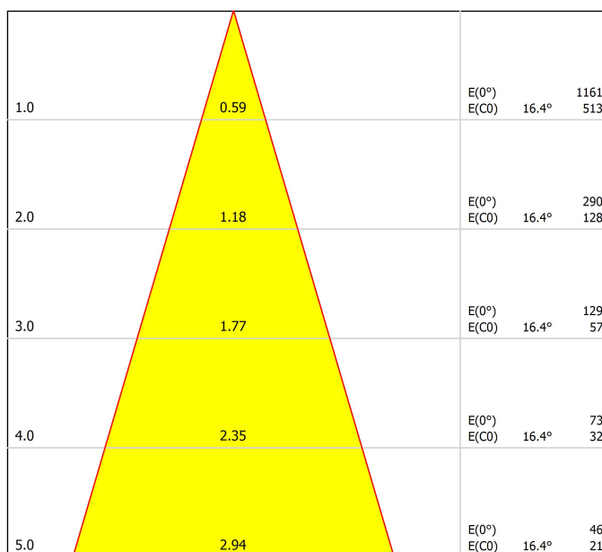
Distance [m] Cone Diameter [m] Illuminance [lx] — C0 - C180 (Half-value Angle: 32.8°)
