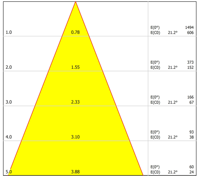
Distance [m] Cone Diameter [m] Illuminance [lx] — C0 - C180 (Half-value Angle: 42.4°)
