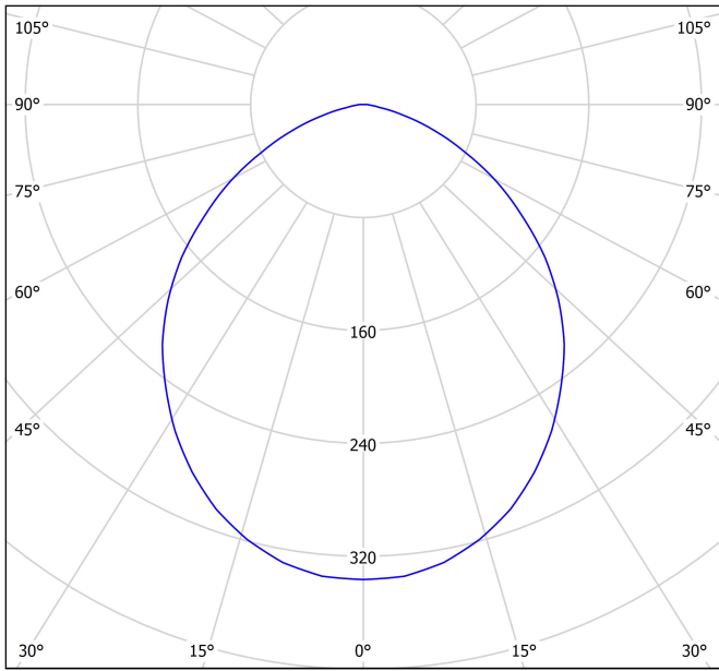
cd/klm — C0 - C180 — C90 - C270 \eta = 80\%
