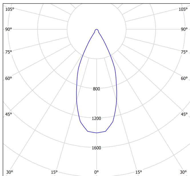
cd/klm — C0 - C180 — C90 - C270 η = 90%
