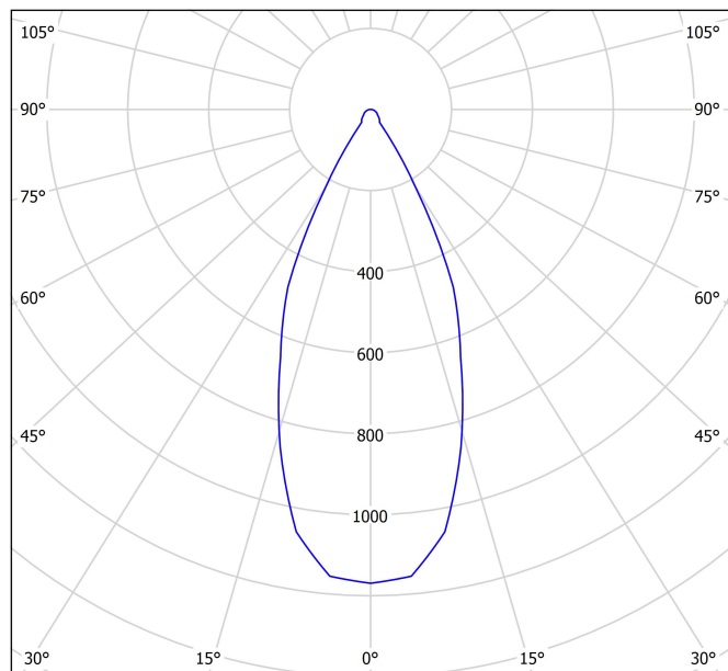
cd/klm — C0 - C180 — C90 - C270 η = 75%
