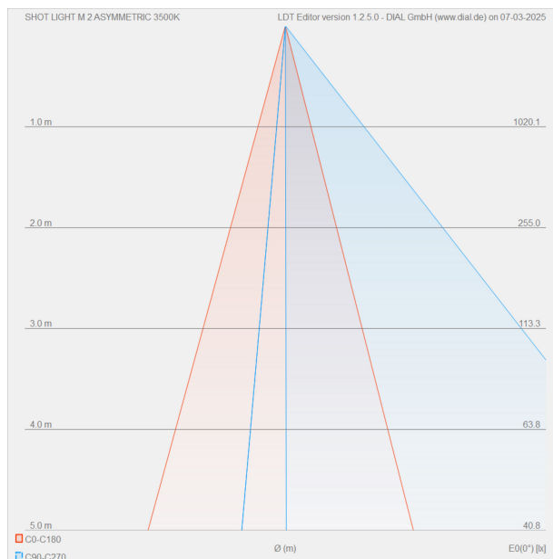
CONICAL DIAGRAM
