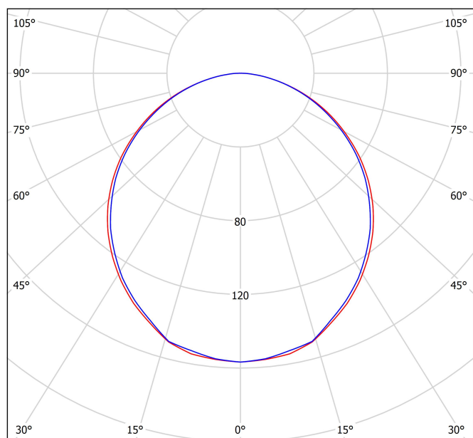
cd/klm — C0 - C180 — C90 - C270 η = 43%
