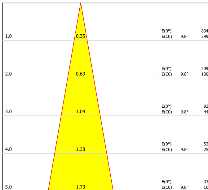
Distance [m] Cone Diameter [m] Illuminance [lx] — C0 - C180 (Half-value Angle: 19.6°)
