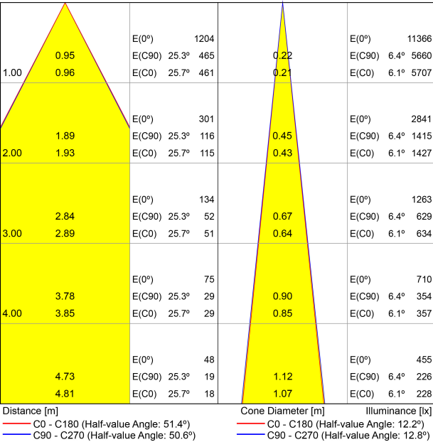
CONICAL DIAGRAM
