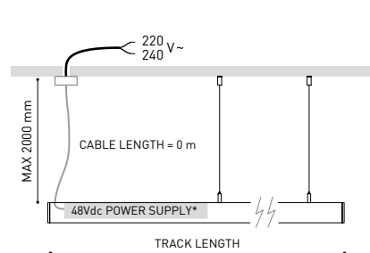
Integrated driver installation
