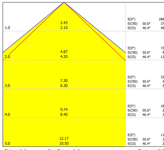
Distance [m] Cone Diameter [m] Illuminance [lx] — C0 - C180 (Half-value Angle: 92.8°) — C90 - C270 (Half-value Angle: 101.2°)
