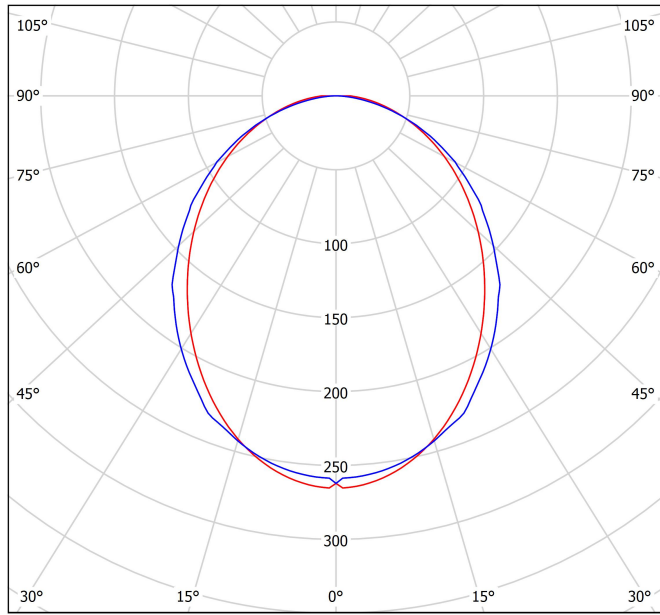
cd/klm \eta = 65\% — C0 - C180 — C90 - C270
