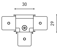
Straight joiner included
