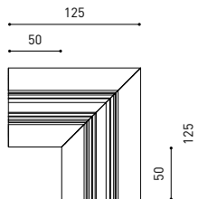
Corner 90° One Plane
