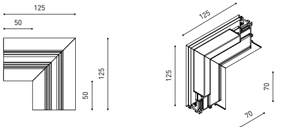
Corner 90° One Plane
