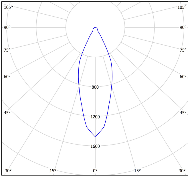
cd/klm \eta = 73\% — C0 - C180 — C90 - C270
