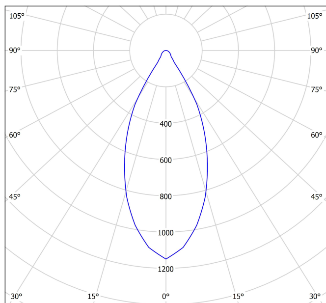
cd/klm — C0 - C180 — C90 - C270 η = 73%
