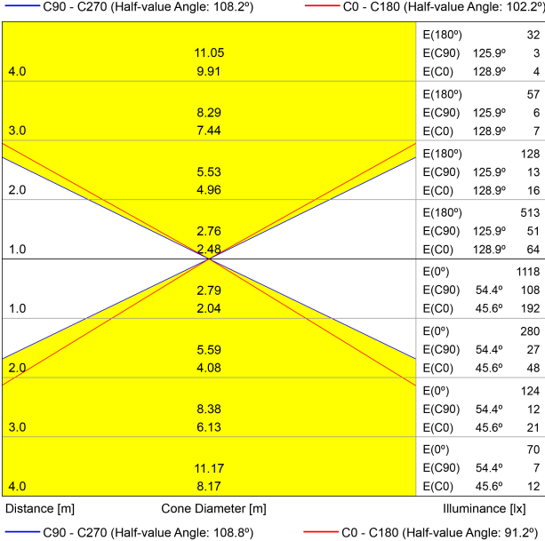
CONICAL DIAGRAM
