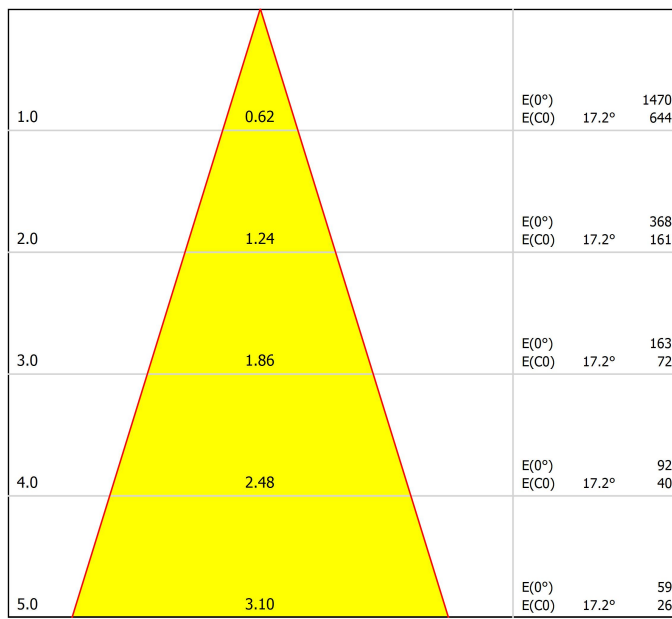
Conical diagram
