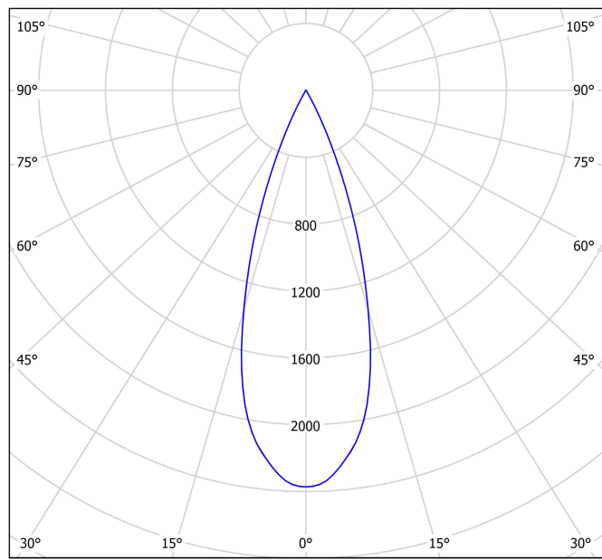
Polar diagram
