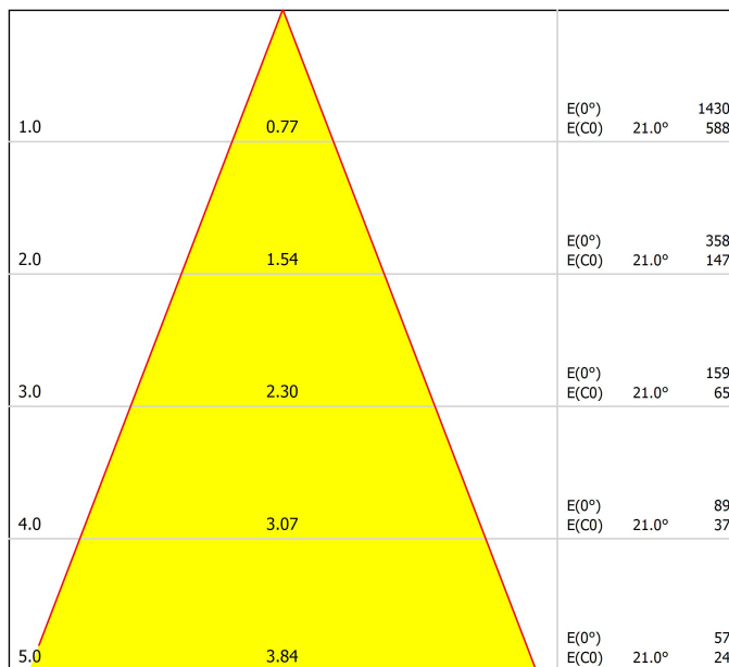
Distance [m] Cone Diameter [m] Illuminance [lx] — C0 - C180 (Half-value Angle: 42.0°)
