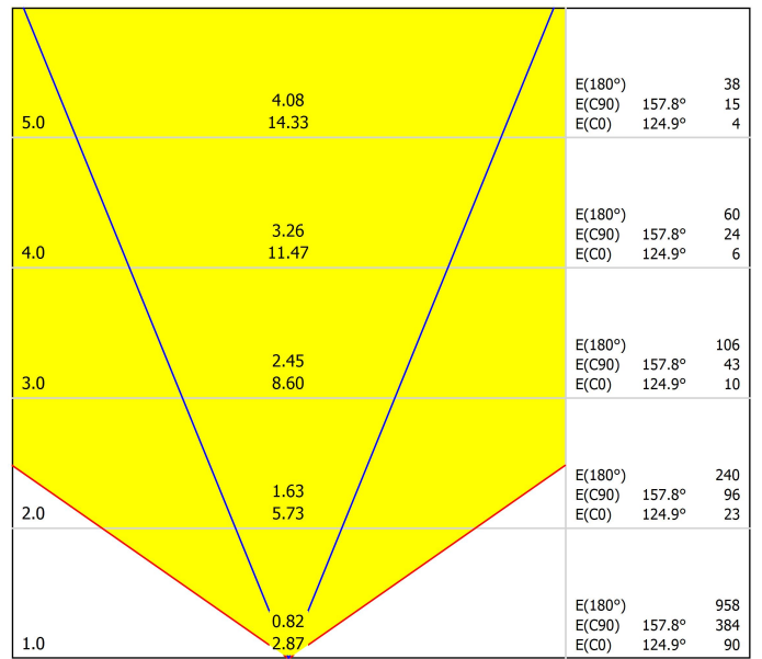
Conical diagram
