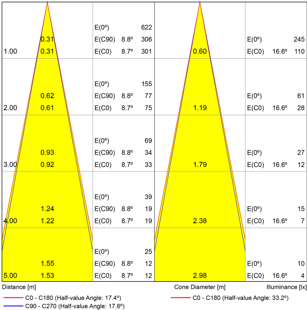
CONICAL DIAGRAM
