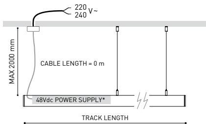
Integrated driver installation
