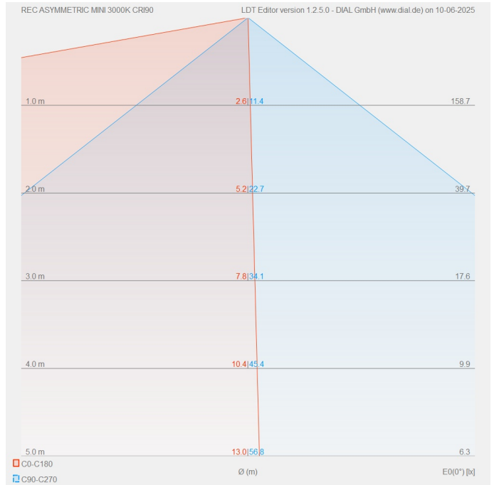
Conical diagram
