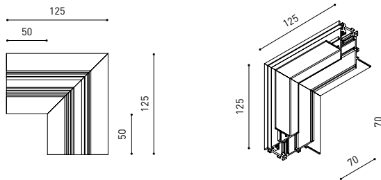
Corner 90° One Plane
