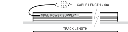
Integrated driver installation
