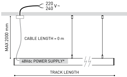
Integrated driver installation
